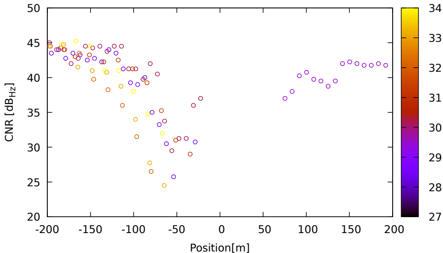
CNR vs position for G04 (L2) on LeicaGS18 - DOY 262 jam. 2
