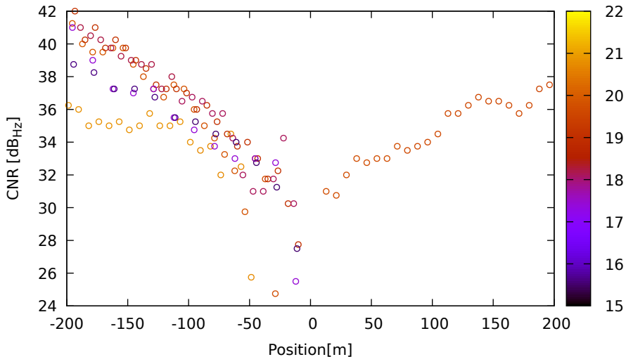
CNR vs position for G08 (L1) on LeicaGS18 - DOY 262 jam. 1
