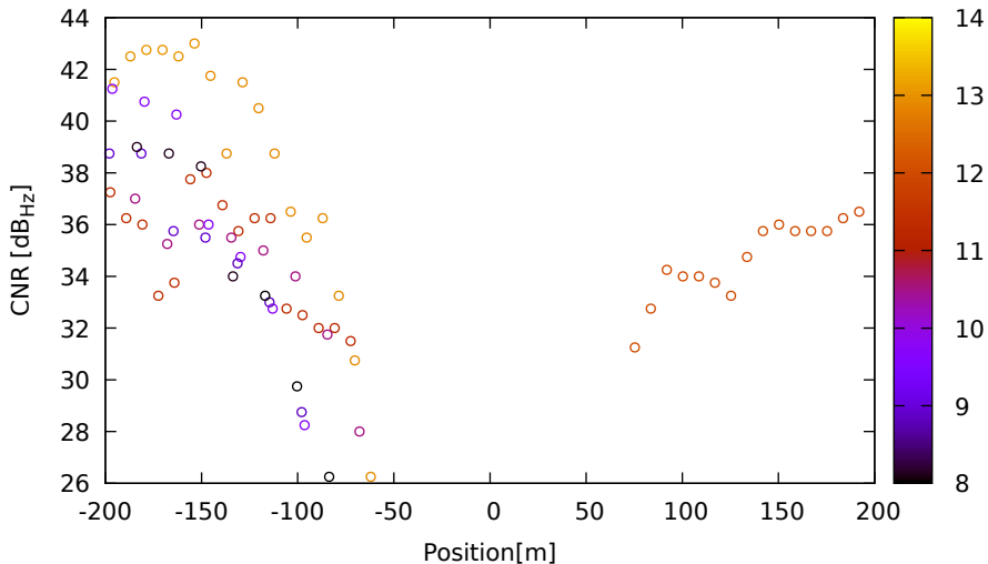
CNR vs position for G08 (L1) on LeicaGS18 - DOY 262 jam. 2
