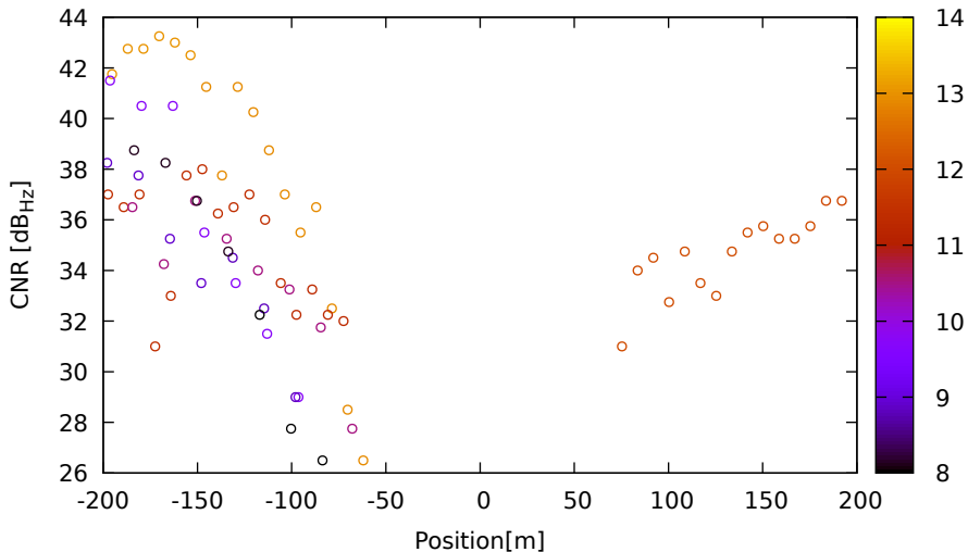
CNR vs position for G08 (L2) on LeicaGS18 - DOY 262 jam. 2
