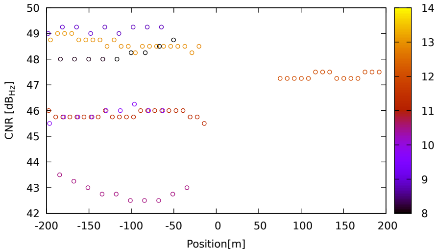
CNR vs position for G08 (L5) on LeicaGS18 - DOY 262 jam. 2
