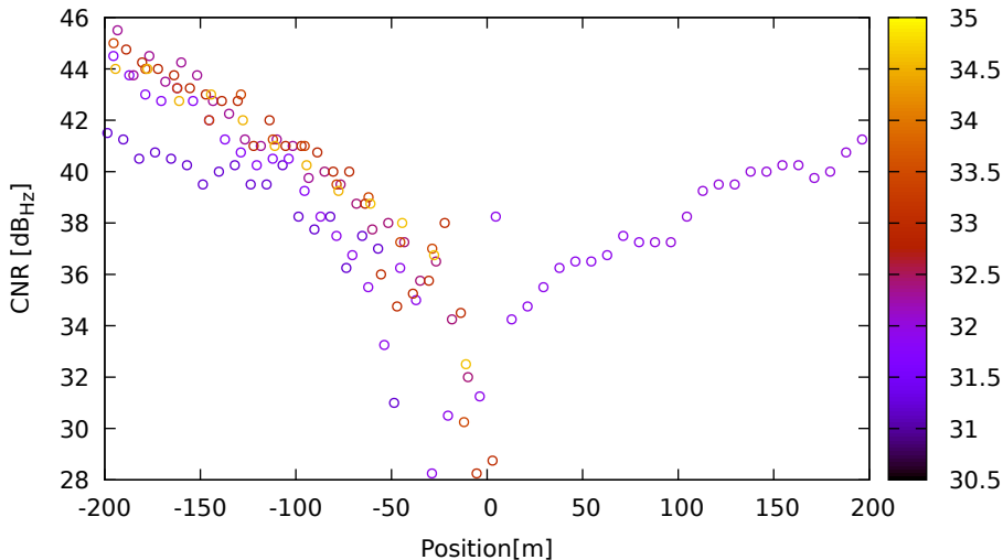
CNR vs position for G17 (L1) on LeicaGS18 - DOY 262 jam. 1
