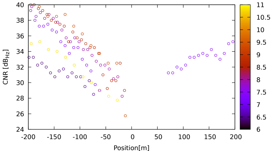
CNR vs position for G19 (L1) on LeicaGS18 - DOY 262 jam. 1
