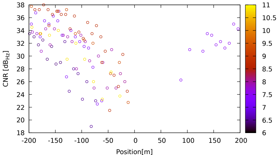
CNR vs position for G19 (L2) on LeicaGS18 - DOY 262 jam. 1
