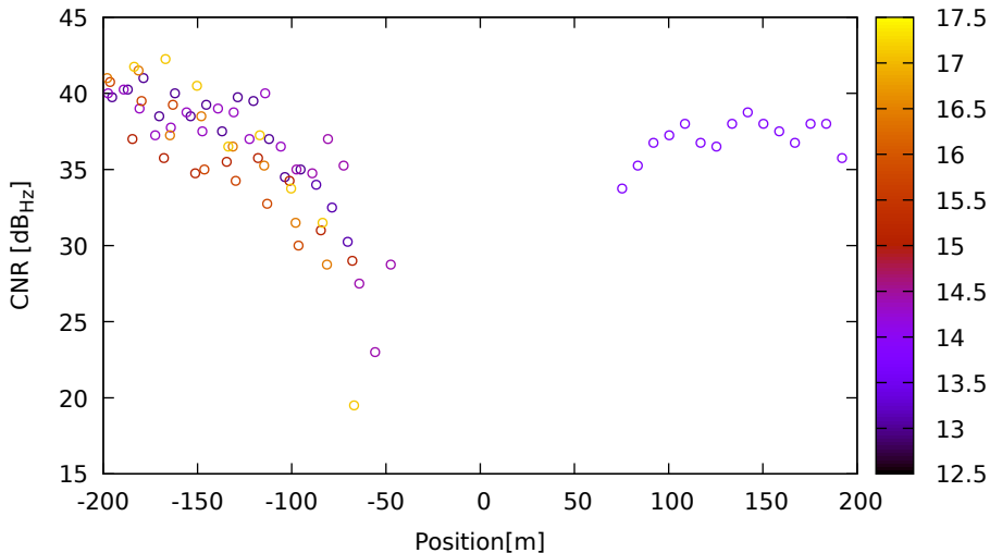
CNR vs position for G19 (L2) on LeicaGS18 - DOY 262 jam. 2
