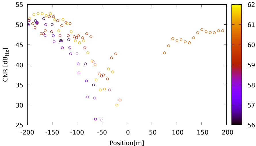
CNR vs position for G21 (L1) on LeicaGS18 - DOY 262 jam. 2
