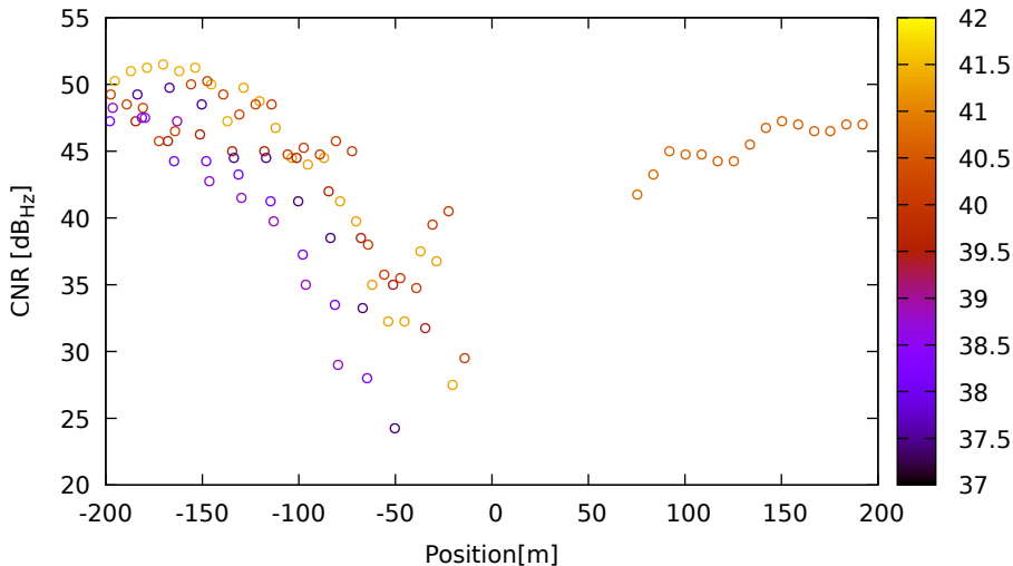
CNR vs position for G22 (L1) on LeicaGS18 - DOY 262 jam. 2
