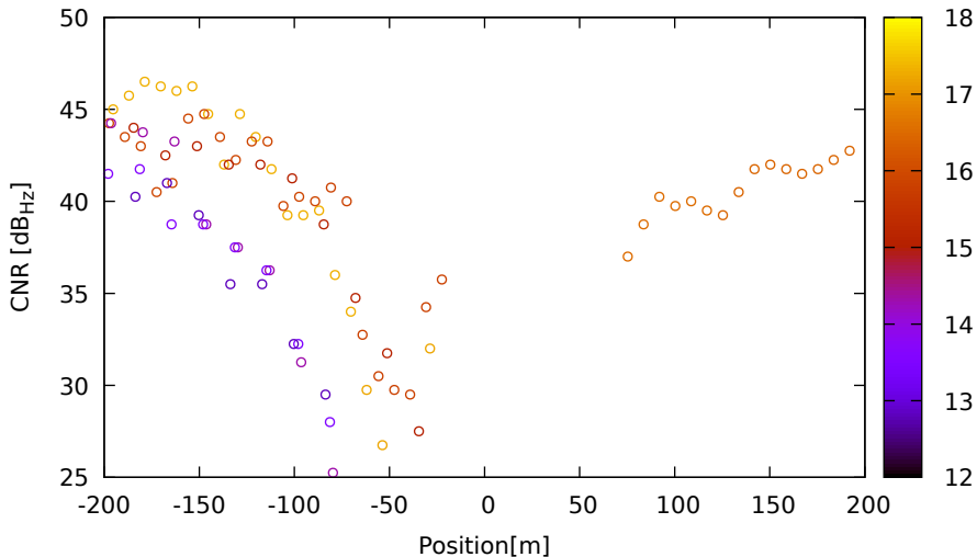
CNR vs position for G32 (L1) on LeicaGS18 - DOY 262 jam. 2
