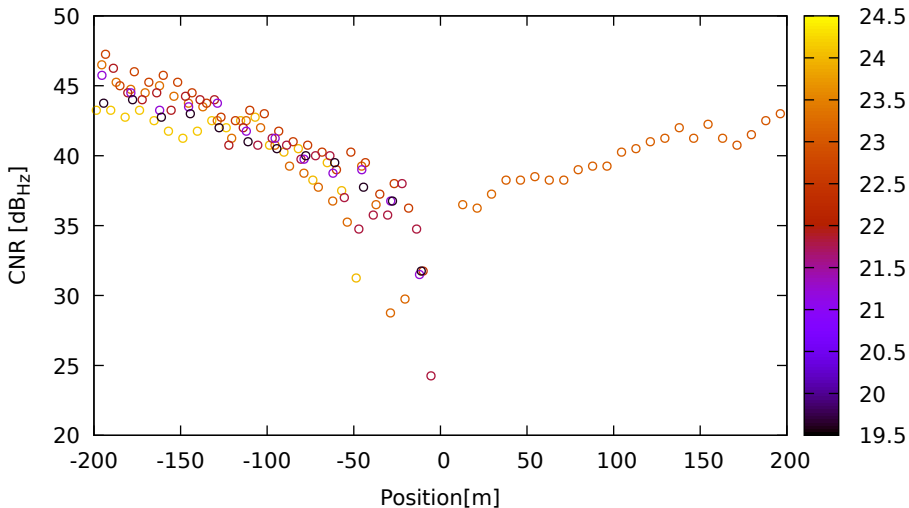
CNR vs position for G32 (L2) on LeicaGS18 - DOY 262 jam. 1
