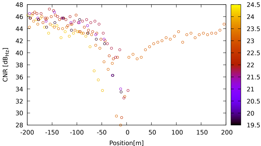
CNR vs position for G32 (L5) on LeicaGS18 - DOY 262 jam. 1
