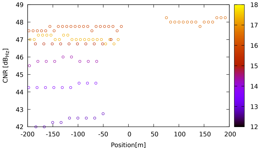
CNR vs position for G32 (L5) on LeicaGS18 - DOY 262 jam. 2
