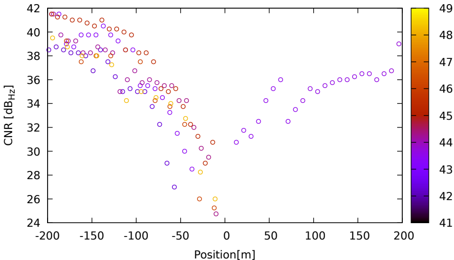
CNR vs position for R01 (G2) on LeicaGS18 - DOY 262 jam. 1
