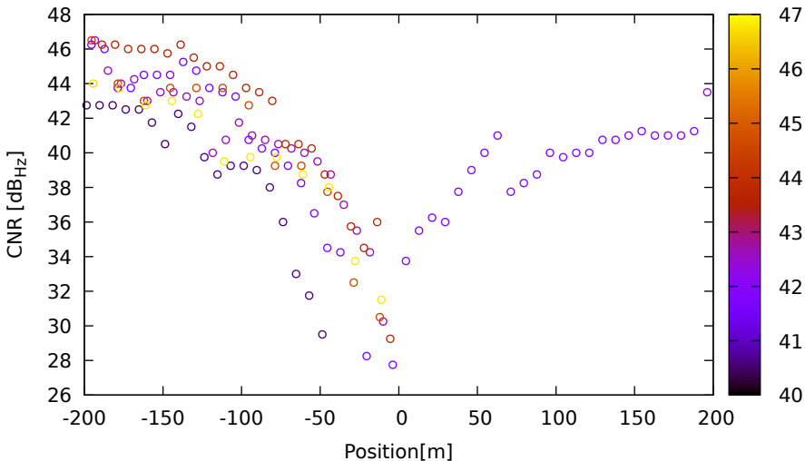
CNR vs position for R24 (G2) on LeicaGS18 - DOY 262 jam. 1
