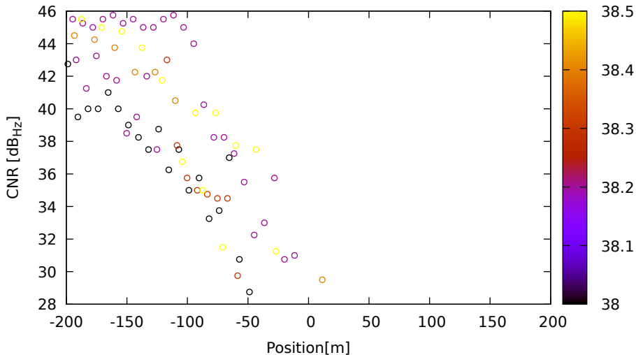
CNR vs position for C09 (B1) on LeicaGS18 - DOY 262 jam. 2
