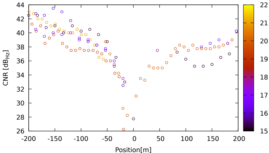
CNR vs position for C11 (B2) on LeicaGS18 - DOY 262 jam. 1
