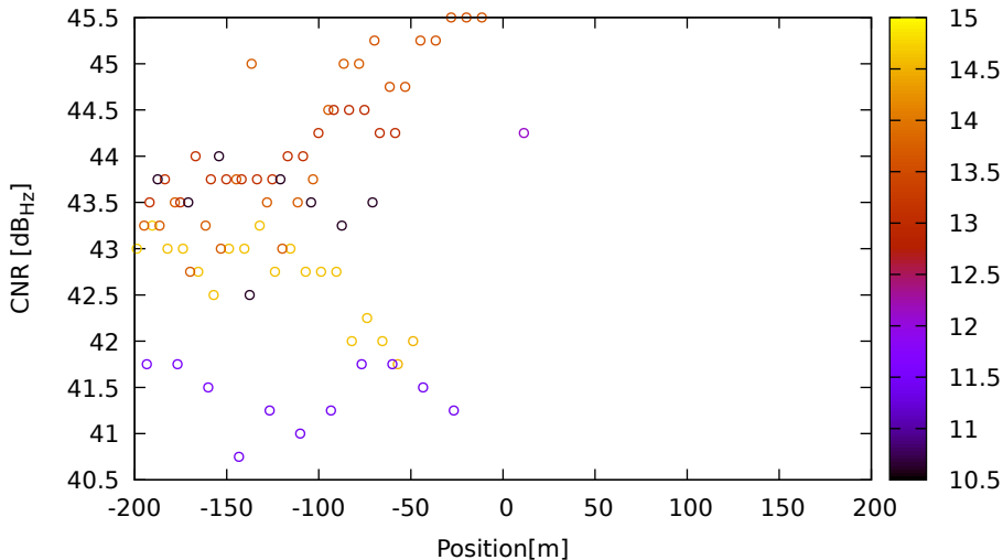
CNR vs position for C11 (B2) on LeicaGS18 - DOY 262 jam. 2
