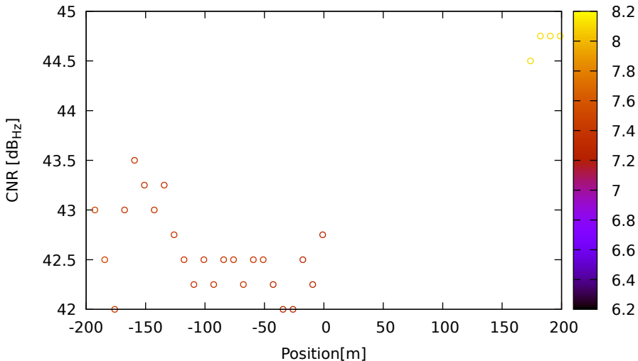
CNR vs position for C11 (B2) on LeicaGS18 - DOY 262 jam. 3
