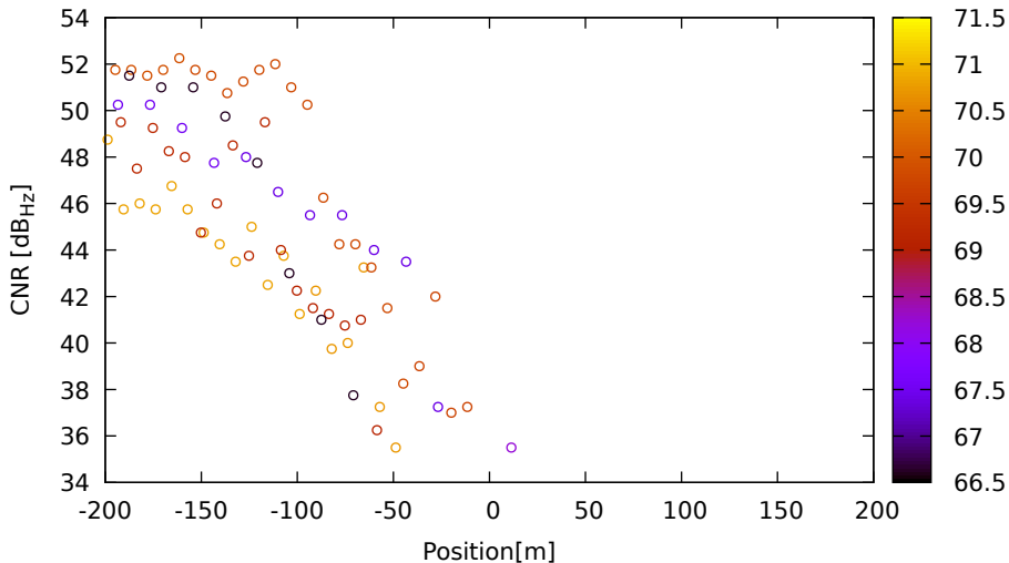
CNR vs position for C14 (B1) on LeicaGS18 - DOY 262 jam. 2
