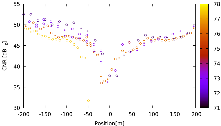
CNR vs position for C14 (B2) on LeicaGS18 - DOY 262 jam. 1
