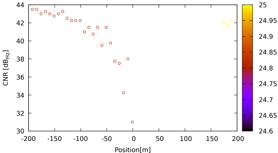
CNR vs position for C16 (B1) on LeicaGS18 - DOY 262 jam. 3
