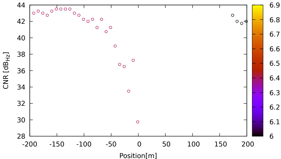
CNR vs position for C26 (B1) on LeicaGS18 - DOY 262 jam. 3
