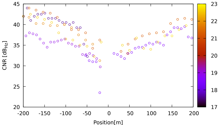
CNR vs position for C27 (B1) on LeicaGS18 - DOY 262 jam. 1
