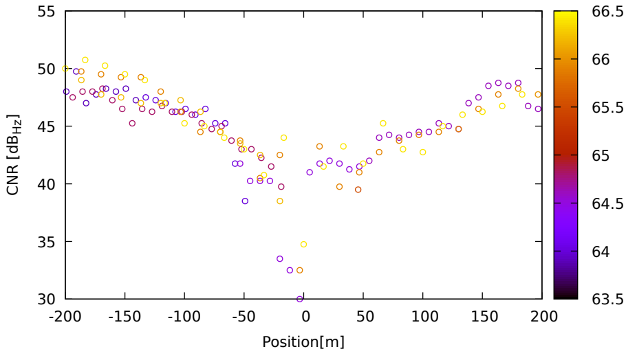
CNR vs position for C28 (B1) on LeicaGS18 - DOY 262 jam. 1
