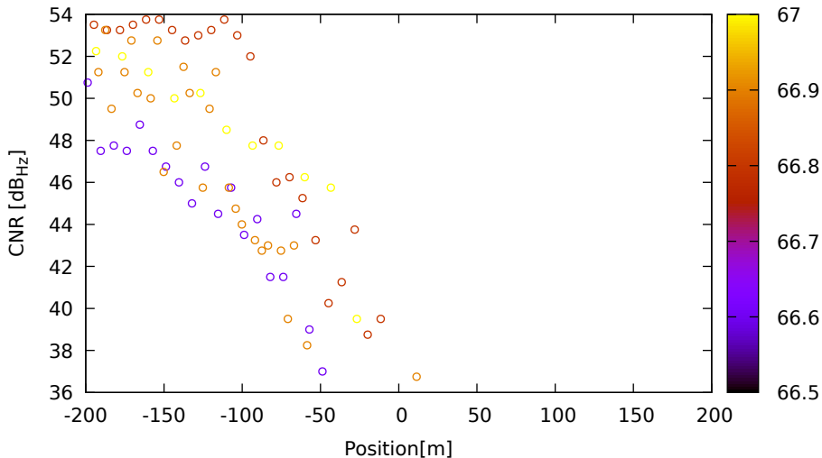
CNR vs position for C28 (B1) on LeicaGS18 - DOY 262 jam. 2
