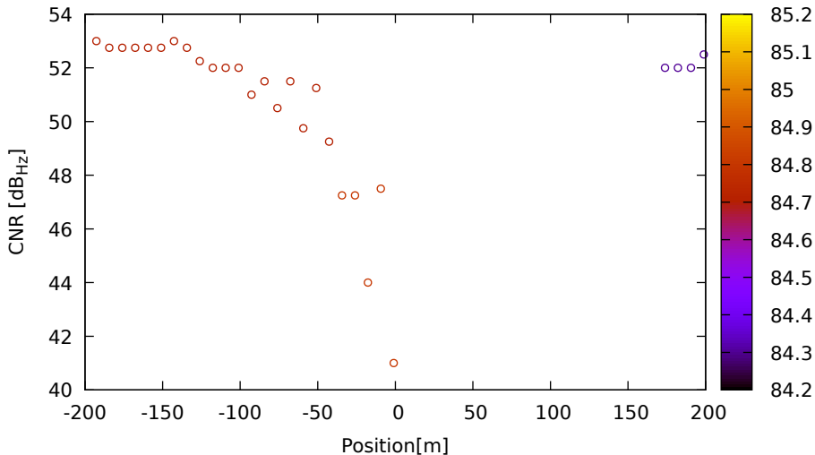
CNR vs position for C33 (B1) on LeicaGS18 - DOY 262 jam. 3
