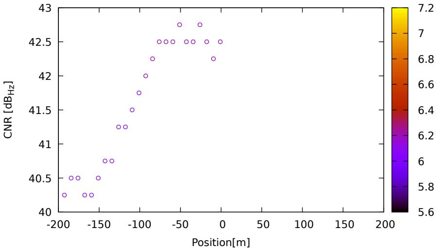
CNR vs position for E03 (E5a) on LeicaGS18 - DOY 262 jam. 3
