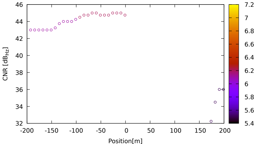
CNR vs position for E03 (E5b) on LeicaGS18 - DOY 262 jam. 3
