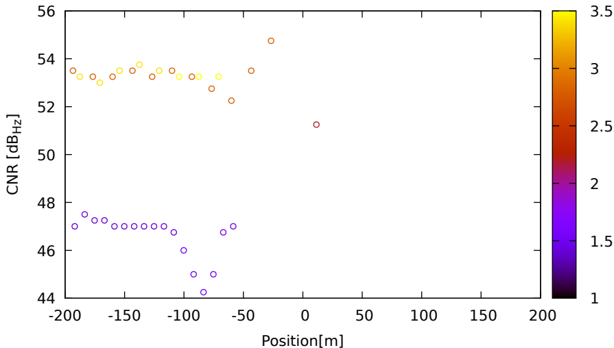
CNR vs position for E03 (E8) on LeicaGS18 - DOY 262 jam. 2
