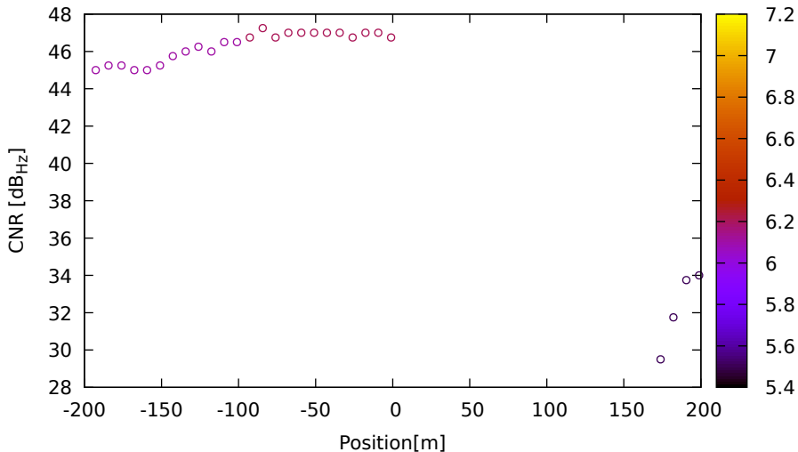
CNR vs position for E03 (E8) on LeicaGS18 - DOY 262 jam. 3
