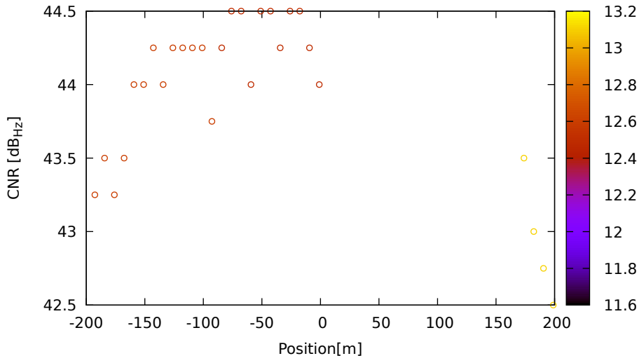
CNR vs position for E04 (E5a) on LeicaGS18 - DOY 262 jam. 3
