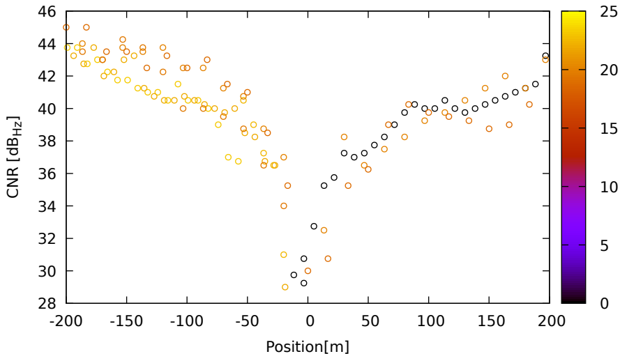
CNR vs position for E04 (E5b) on LeicaGS18 - DOY 262 jam. 1
