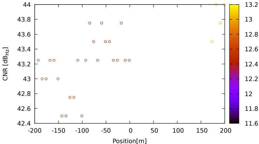
CNR vs position for E04 (E5b) on LeicaGS18 - DOY 262 jam. 3
