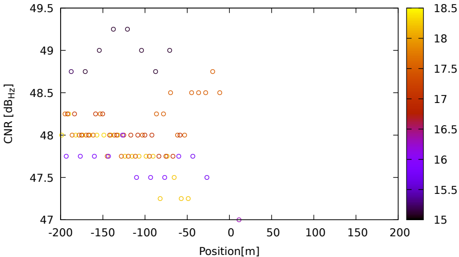
CNR vs position for E04 (E8) on LeicaGS18 - DOY 262 jam. 2
