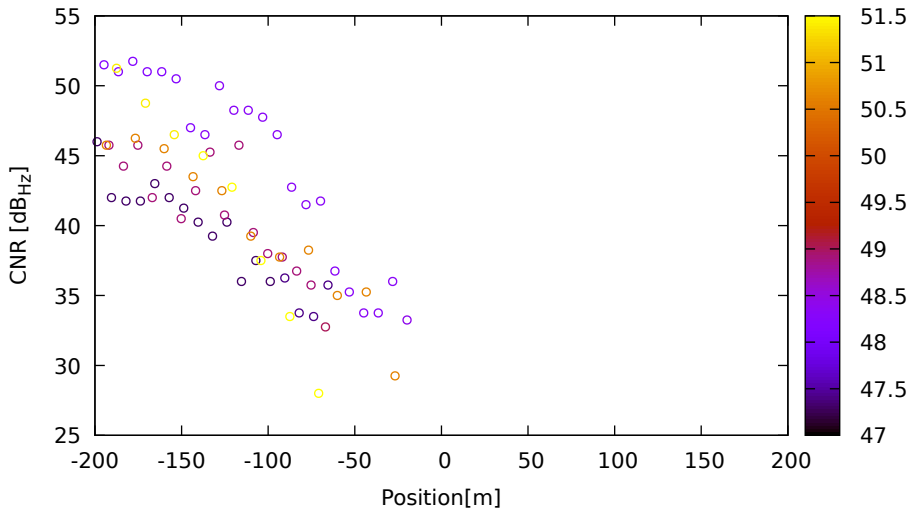
CNR vs position for E05 (E1) on LeicaGS18 - DOY 262 jam. 2
