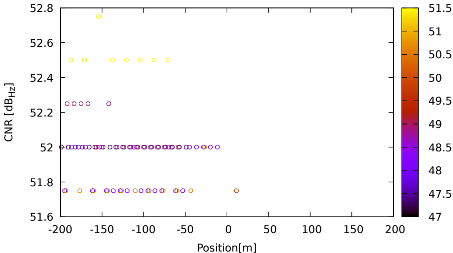
CNR vs position for E05 (E5a) on LeicaGS18 - DOY 262 jam. 2
