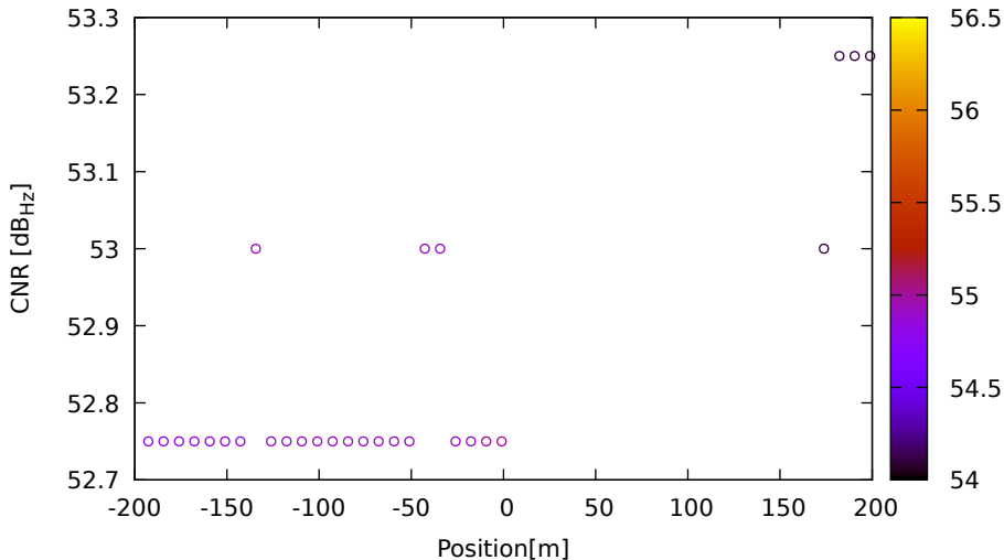
CNR vs position for E05 (E5a) on LeicaGS18 - DOY 262 jam. 3
