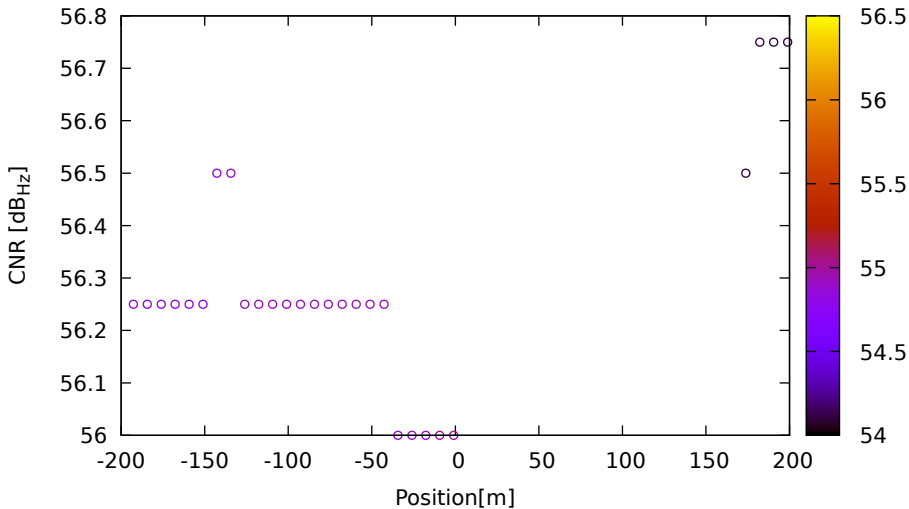
CNR vs position for E05 (E8) on LeicaGS18 - DOY 262 jam. 3
