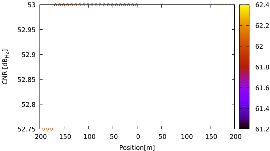
CNR vs position for E09 (E5a) on LeicaGS18 - DOY 262 jam. 3
