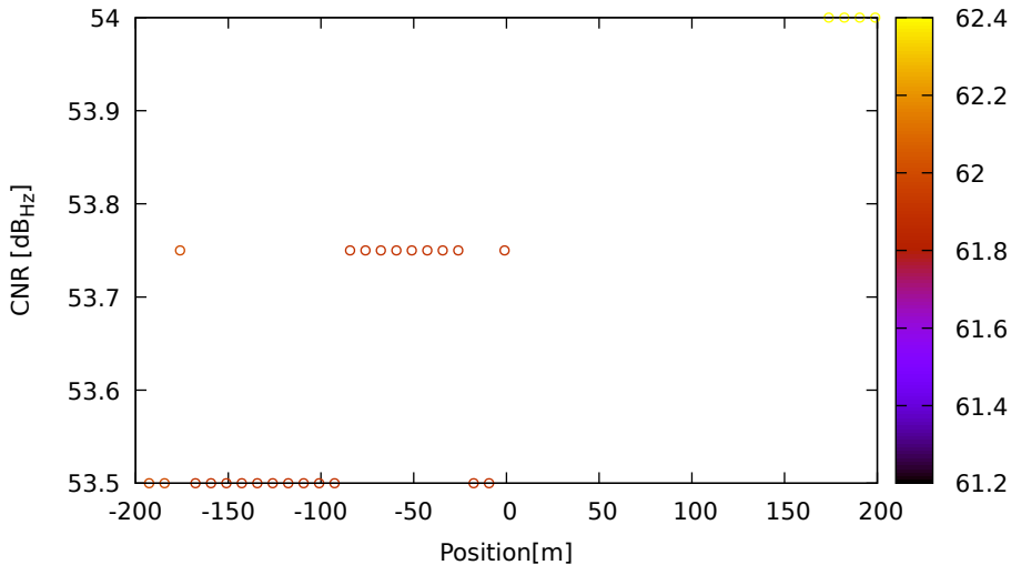
CNR vs position for E09 (E5b) on LeicaGS18 - DOY 262 jam. 3
