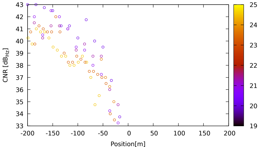
CNR vs position for E11 (E5a) on LeicaGS18 - DOY 262 jam. 1
