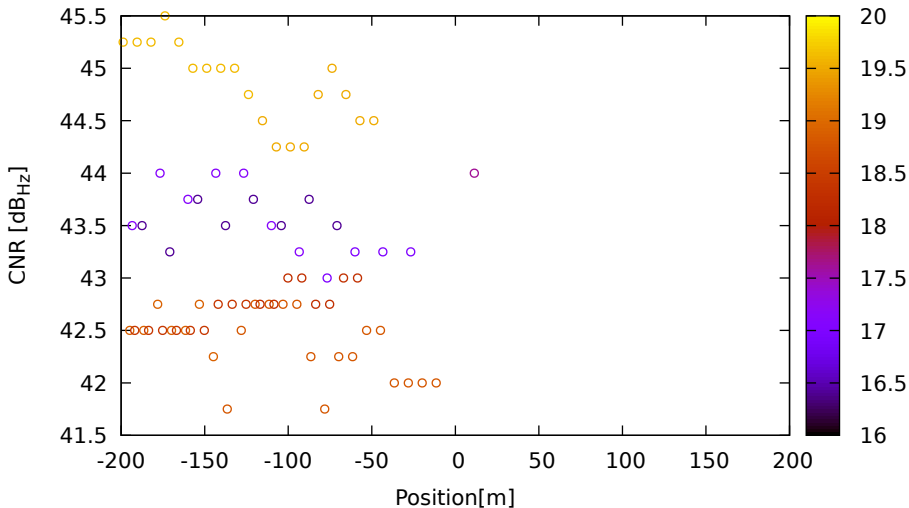
CNR vs position for E11 (E5a) on LeicaGS18 - DOY 262 jam. 2
