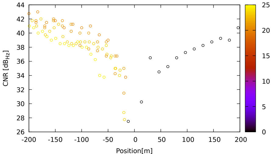
CNR vs position for E11 (E5b) on LeicaGS18 - DOY 262 jam. 1
