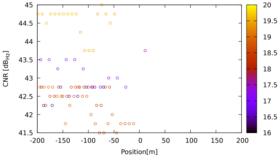
CNR vs position for E11 (E5b) on LeicaGS18 - DOY 262 jam. 2
