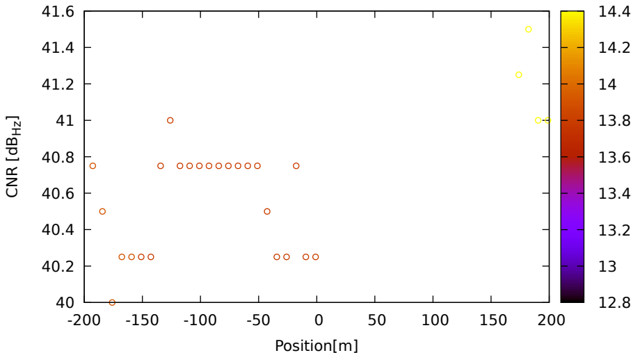
CNR vs position for E11 (E5b) on LeicaGS18 - DOY 262 jam. 3
