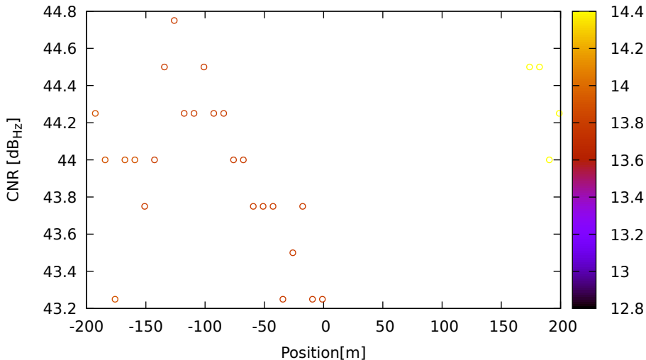
CNR vs position for E11 (E8) on LeicaGS18 - DOY 262 jam. 3
