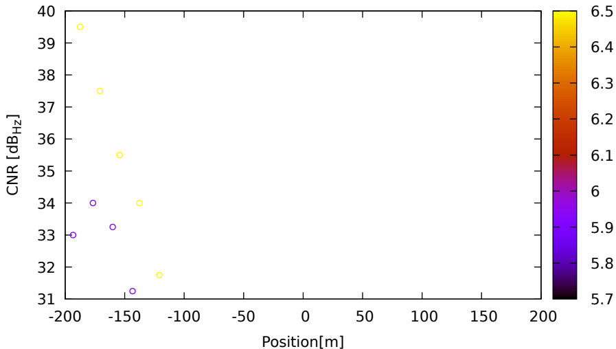
CNR vs position for E15 (E1) on LeicaGS18 - DOY 262 jam. 2
